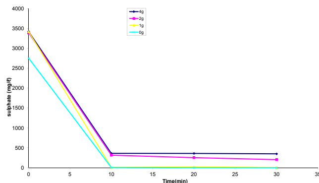
Figure 3 Effect of \text{BaSO}_4 seed crystals on the removal rate of sulphate
