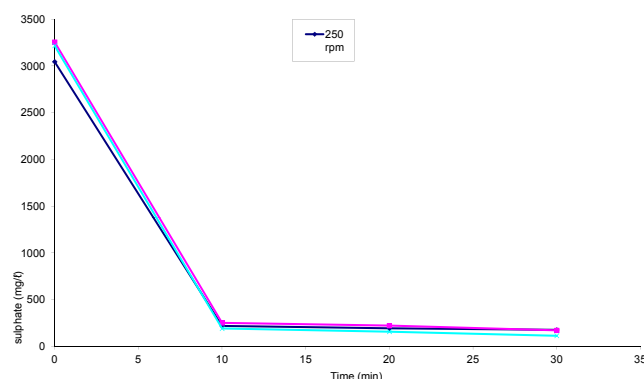
Figure 4 Effect of stirring rate on the removal rate of sulphate
