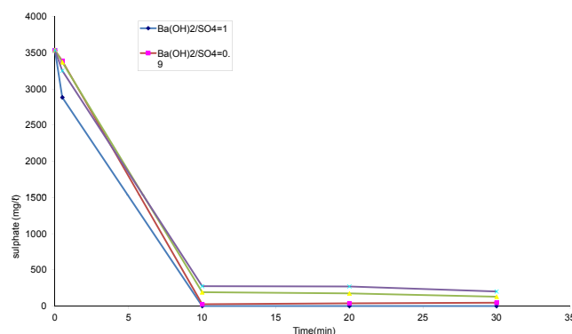
Figure 2 Effect of \text{Ba}(\text{OH})_2/\text{SO}_4 mole ratio on the removal rate of sulphate
